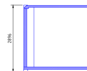
SIDE SECTION
